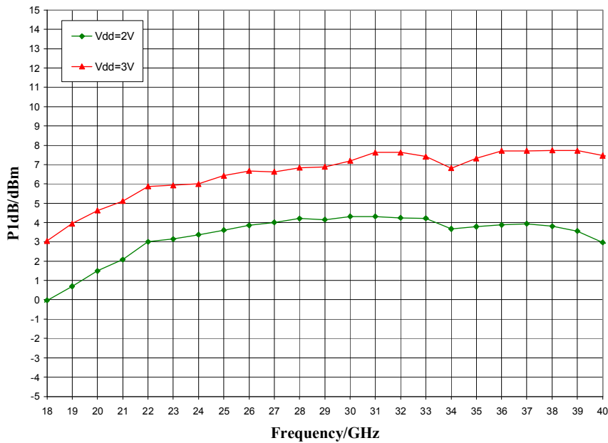
P1dB vs. V_{dd} , V_{gg} = 3.0\text{ V} , T_A = 25\text{ }^\circ\text{C}
