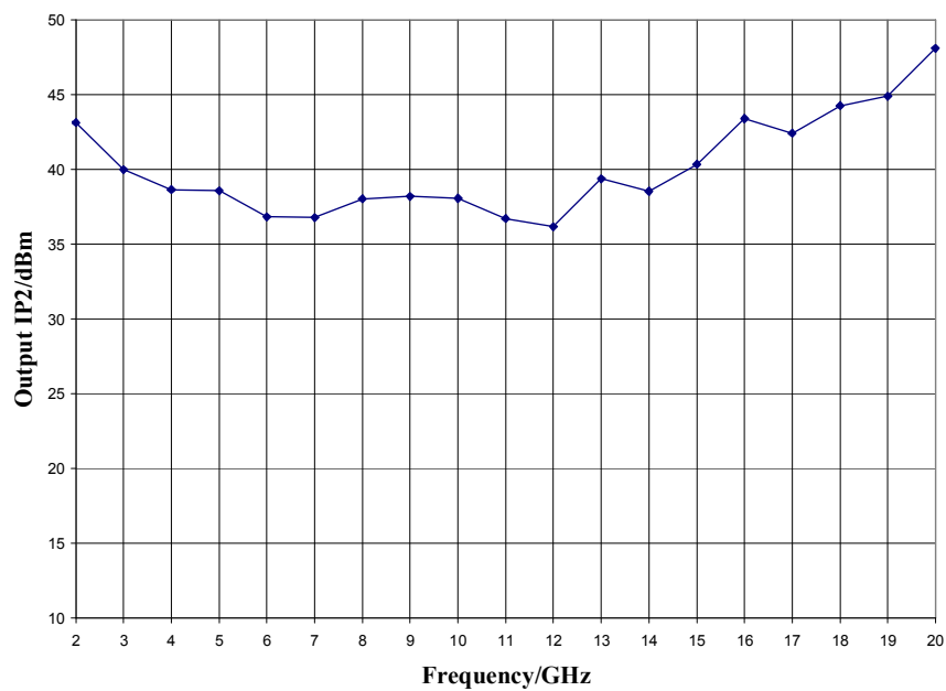
Output IP2, V_{dd} = 5.0\text{ V} , I_{dd} = 74\text{ mA} , T_A = 25\text{ }^\circ\text{C}
