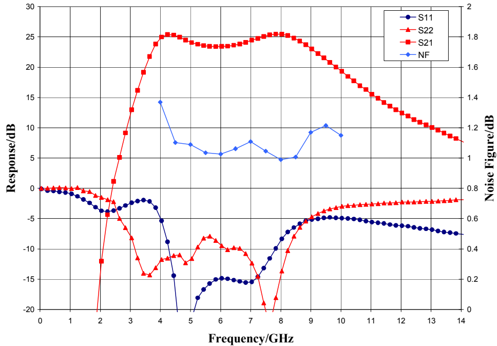
Narrow-band Performance, V_{dd} = 10\text{ V} , V_{gg} = -2.3\text{ V} , I_{dd} = 75\text{ mA} , T_A = 25\text{ }^\circ\text{C}
