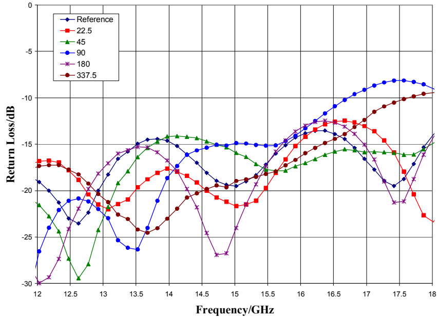
Output Return Loss, Major States, T_A = 25\text{ }^\circ\text{C}
